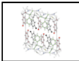
Fig. 2. A part of the crystal packing of the crystal structure of 3-chlorobenzylammonium phenylmalonate dihydrate, viewed down the b axis showing a network of hydrogen bonds. Hydrogen bonds are shown by broken lines. Colour codes for residues: RED & BLACK = 3-chlorobenzylammonium; GREEN = phenylmalonate; BLUE & YELLOW = water molecules.
